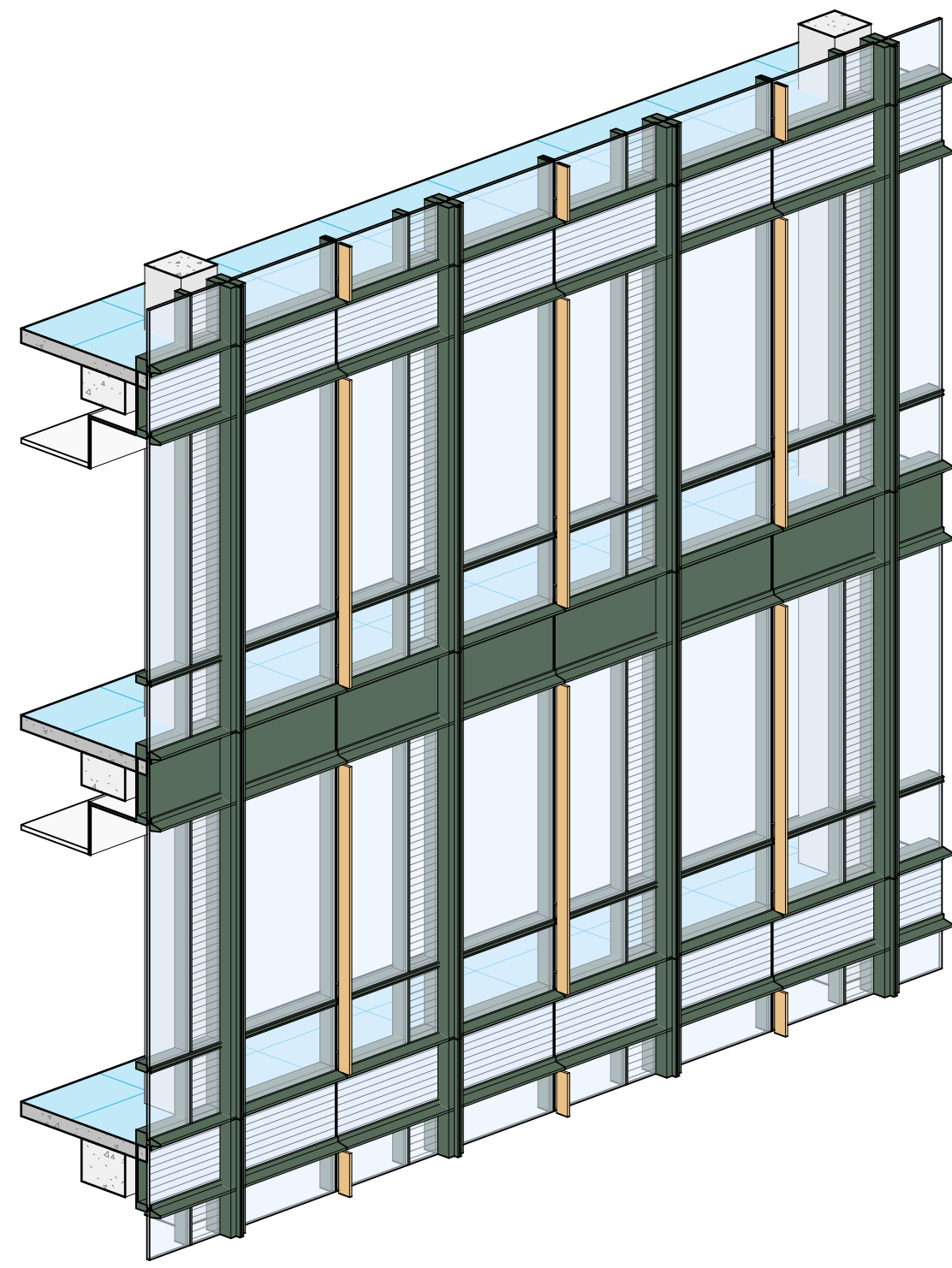
1 ENCLOSURE TYPE A1
