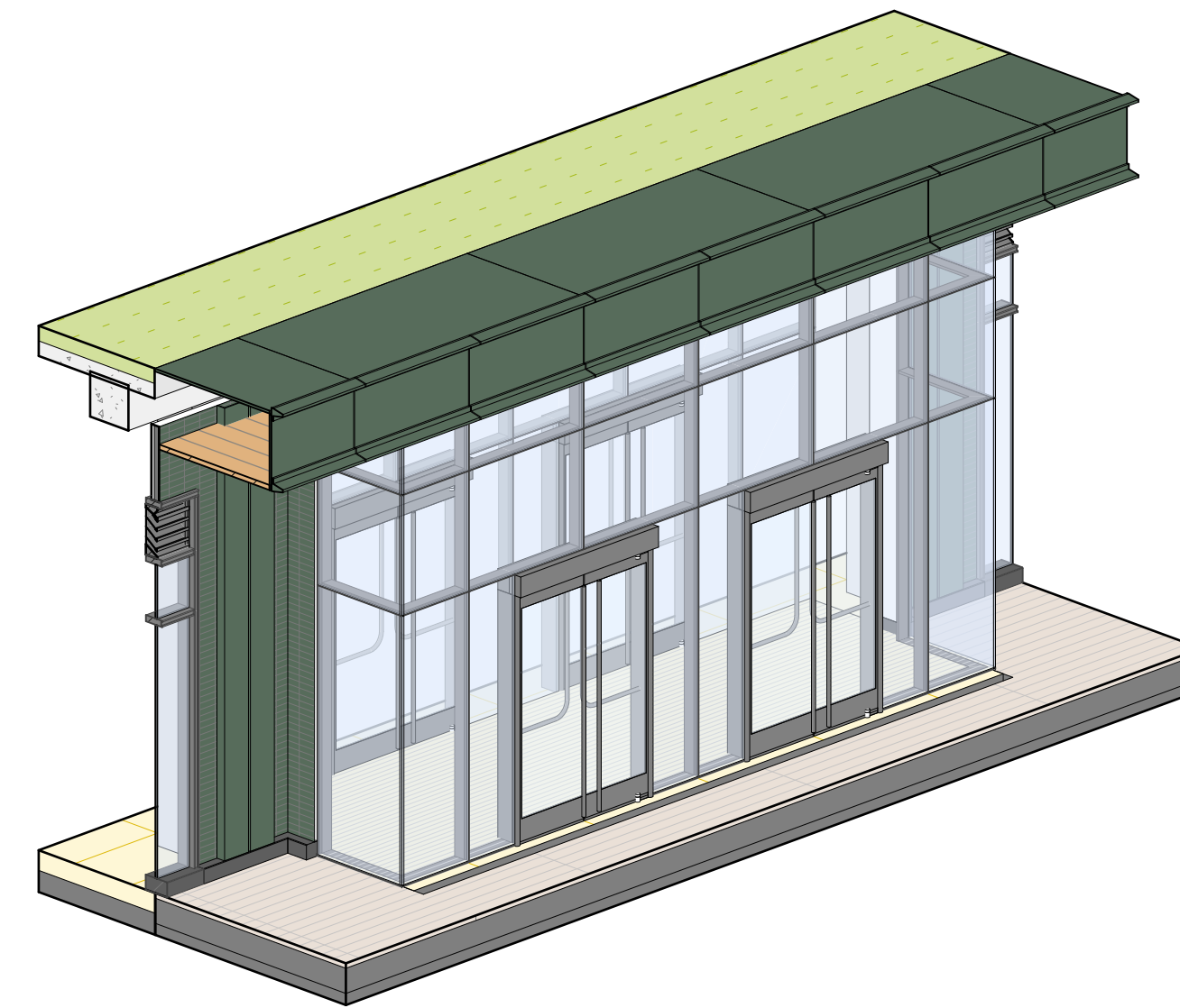
10 ENCLOSURE TYPE D3
