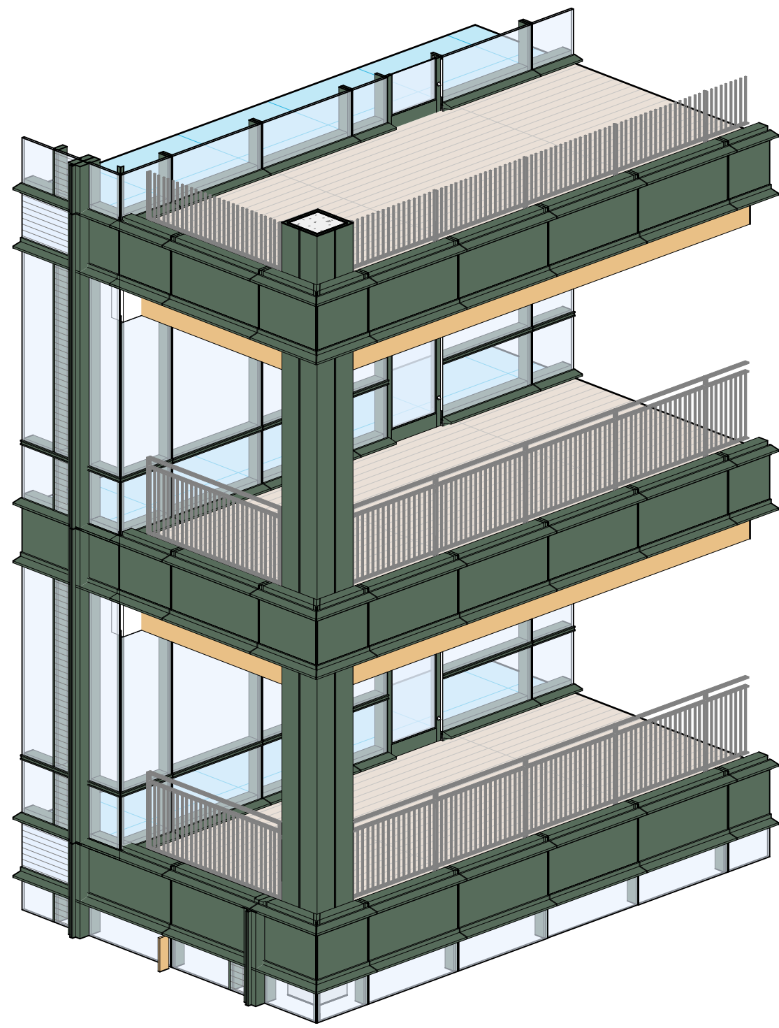
2 ENCLOSURE TYPE A2
